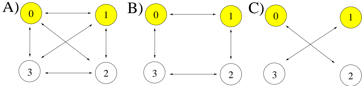
Figure 3: Three possible architectures with single arrows leading to a balanced coloring in a ring with the synchrony pattern described in the text. From left to right A) a_1 = a_2 = a_3 = 1 , B) a_1 = a_3 = 1, a_2 = 0 , C) a_1 = a_3 = 0, a_2 = 1 . In all cases a_0 = 0 , corresponding to no self-coupling.
