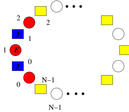
Figure 6: A ring network with two cell types, E and I. Cells of each type are numbered from 0 up to N - 1 , increasing in the clockwise direction, and each cell population is subdivided into two clusters, as shown.
