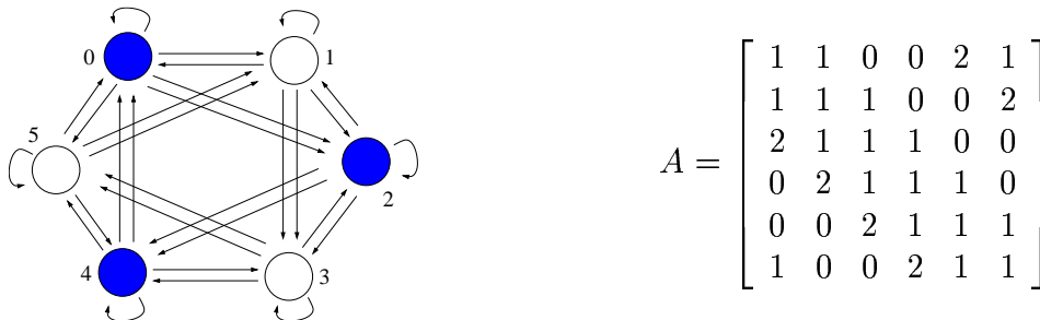
Figure 2: An example of a network of six identical cells and its connectivity matrix.
