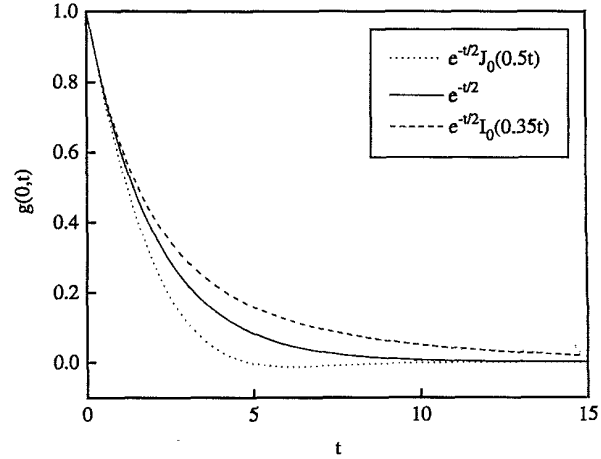
FIG. 3. Three representative response functions corresponding to the parameters: \nu = 0.25 , \beta = 1 , and \alpha = 0.5 (dotted line), \alpha = 0.25 (solid line), \alpha = 0.128 (dashed line).
