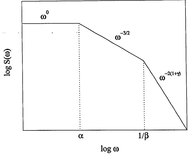
FIG. 2. The form (not to scale) of the autocorrelation function S(\omega, z = 0) in the frequency domain for the pinned polymer model.
