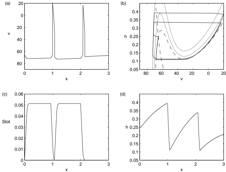
FIG. 12. Various perspectives of a two-pulsed solution, which was found for \gamma \approx 0.1 (in general, multipulsed waves can be generated at small values of \gamma ): (a) Plot of v versus x . (b) Projection of solution trajectory (double-looped solid curve) onto the (v, h) phase plane; the dashed curves are the nullclines for S_{tot} = 0 , the dotted curve is the cubic-shaped nullcline for S_{tot} \approx 0.0186 , and the dot-dashed curve corresponds to the cubic-shaped nullcline for S_{tot} \approx 0.0515 . (c) Plot of S_{tot} versus x . (d) Plot of h versus x .
